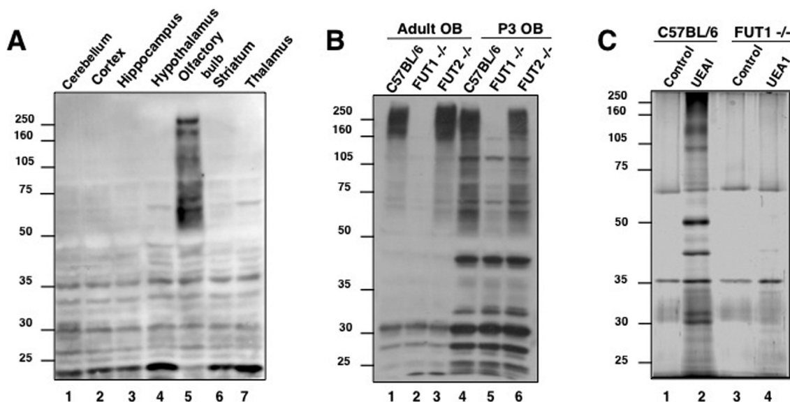
FIGURE 1: Fuc \alpha (1–2)Gal glycoproteins are enriched in mammalian OB, and their expression is regulated by FUT1. (A) Fuc \alpha (1–2)Gal glycoproteins are highly expressed in the adult rat OB relative to other brain regions. (B) Comparison of glycoproteins present in wild-type C57BL/6, FUT1-deficient, and FUT2-deficient mouse OBs from adult and P3 mouse brain tissue. Fuc \alpha (1–2)Gal glycoproteins were detected with UEA1 conjugated to horseradish peroxidase. An equal amount of protein (200 \mu g) was loaded in each lane. (C) Silver-stained gel of Fuc \alpha (1–2)Gal proteins isolated by UEA1 lectin affinity chromatography from the OBs of P3 wild-type C57BL/6 and FUT1-deficient animals.
